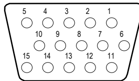
VGA/SVGA connector (Model 75E, rear panel)
